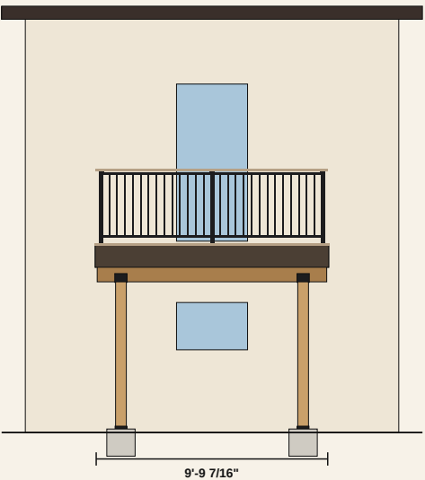
FRONT ELEVATION — from the yard
